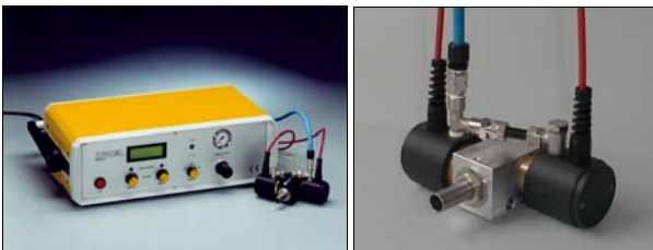
Electrostatic Aerosol Neutralizer EAN 581 (le); Mixing chamber with ionization heads (ri)
