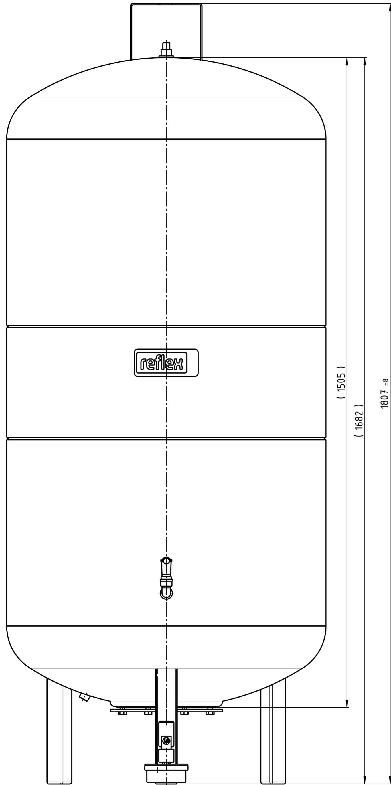
Front view
