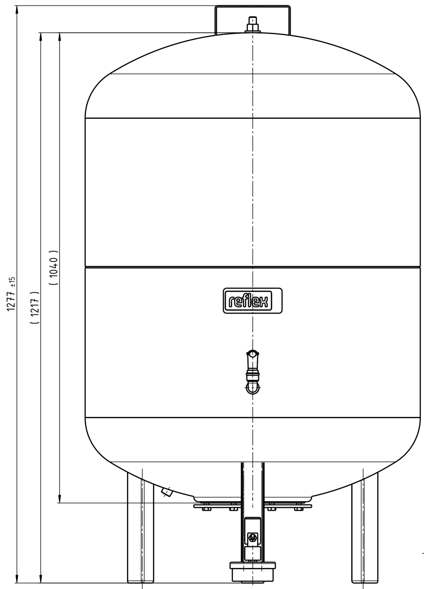
Front view
