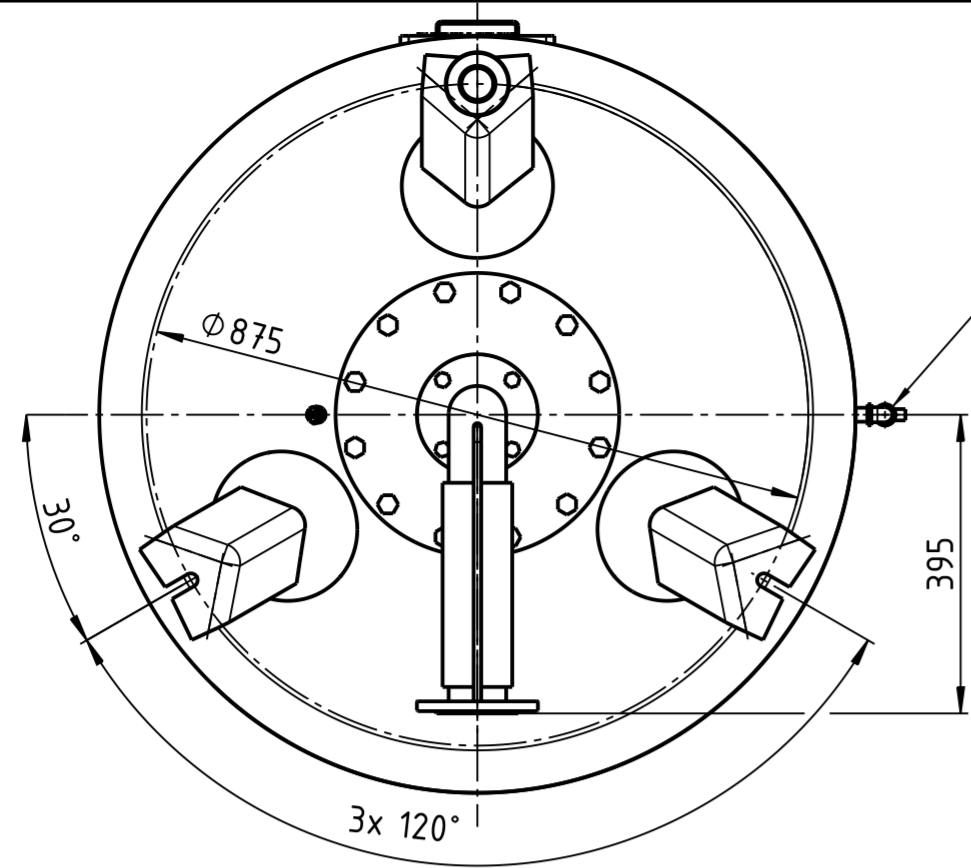
Bottom view
