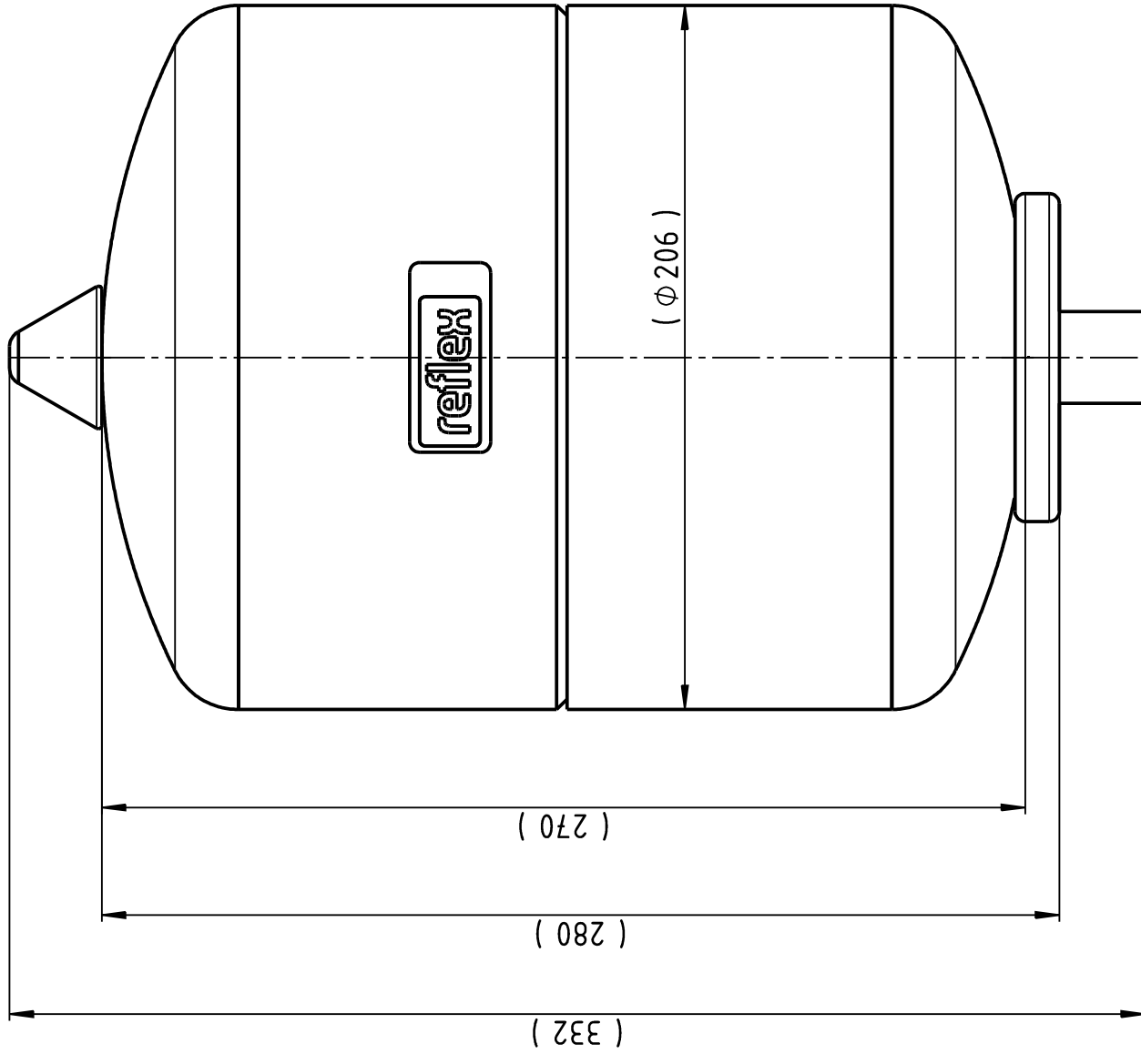
Front view
