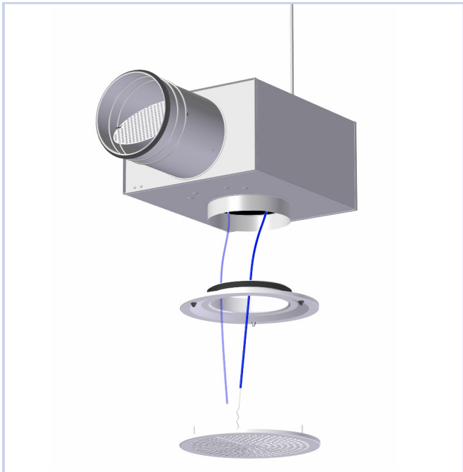
Fig. 5: Installation
