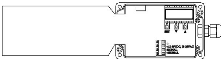
Figure 2: Inside of Electronic Enclosure
